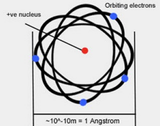
Nuclear Model
