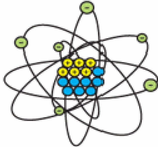
C-14 Unstable
