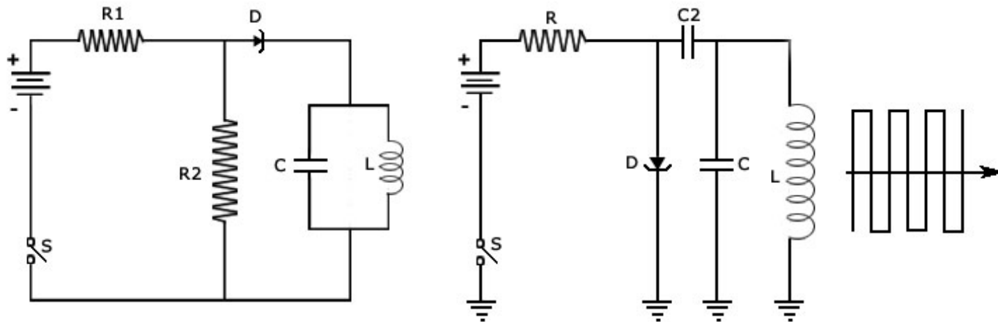
TUNNEL DIODE OSCILLATOR CIRCUIT
