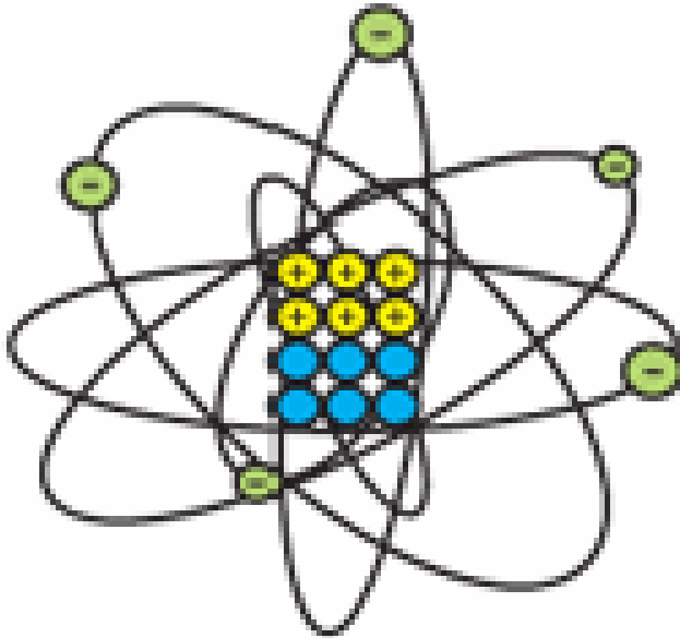
C-12 Stable
